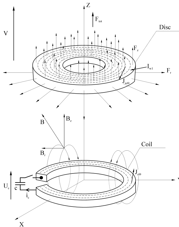
Fig. 3. IDD-System of coaxial inductor (coil) and disc.
