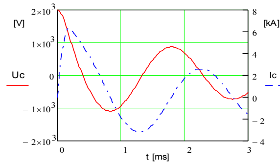
Fig.5. Capacitor voltage and coil current (Fig.3).
