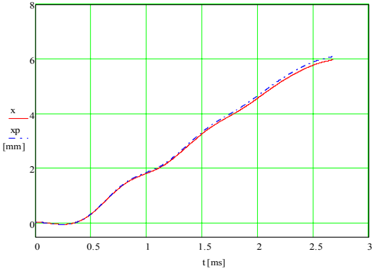
Fig.24. The comparison of the obtained characteristics from the optimizer ( x ) and the potentiometer ( x_p ).
