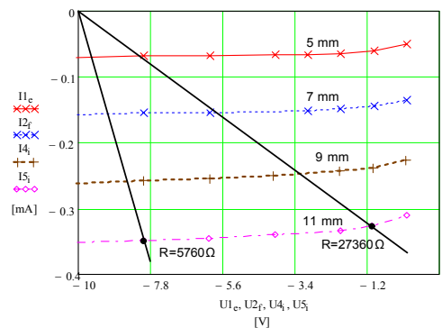
Fig. 15. The photo-diode characteristics.
