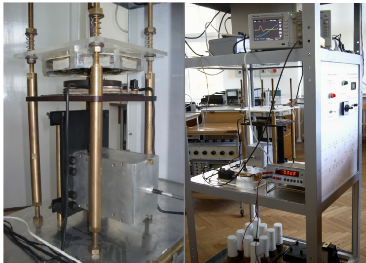
Fig. 18. The optimeter connected with IDD and the measuring system.
