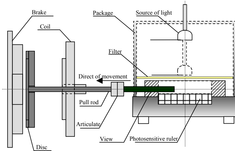
Fig. 13. Construction of the measuring system of displacement.
