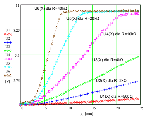
Fig. 17. The characteristics of the voltage in the displacement function U=f(X) for a lamp of 3.2W at different loads.
