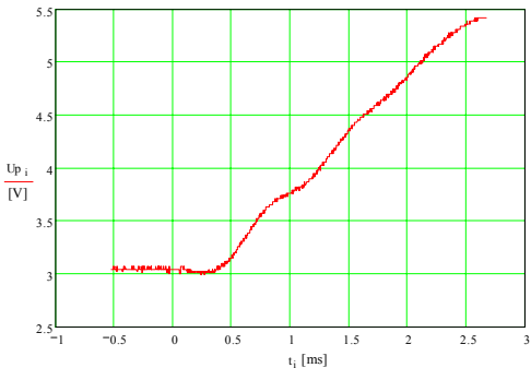
Fig. 21. The U(t) characteristics of potentiometer.
