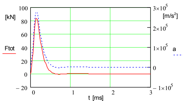
Fig. 9. Resultant force and acceleration.
