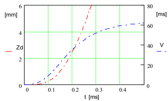
Fig. 7. Enlargement of box for Fig.6.
