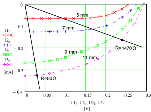
Fig. 14. The current-voltage characteristics of the photo-voltaic cell.
