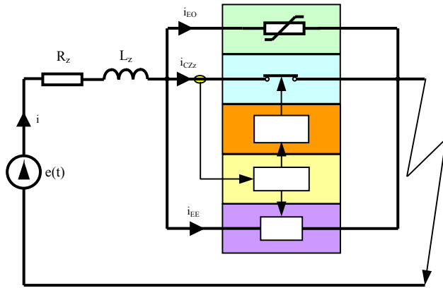
Fig. 1. Scheme of HB in short-circuit.
