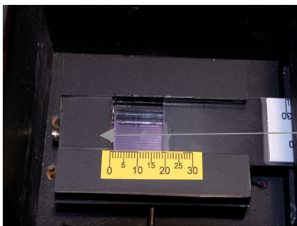
Fig. 11. The view of “a photosensitive ruler” with a diaphragm.
