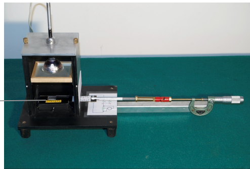
Fig. 12. The external view of an optimizer.
