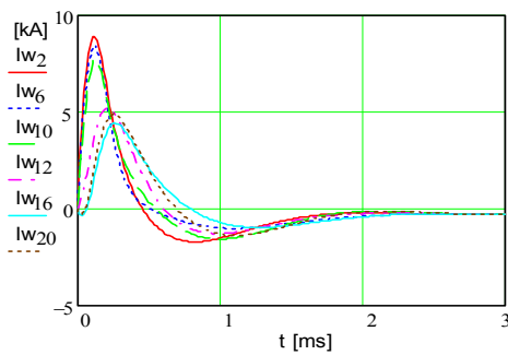
Fig.4. Disc currents in few filaments (Fig.3).
