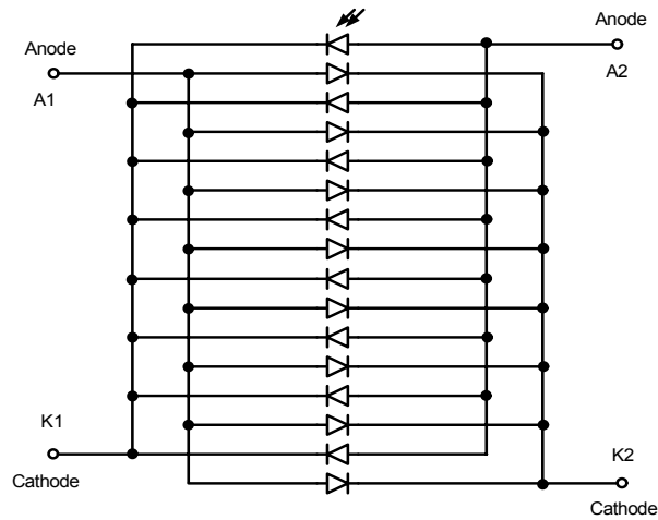
Fig. 10. Photosensitive ruler- photoelements connected in parallel.
