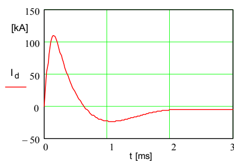
Fig. 8. Entire current of disc.
