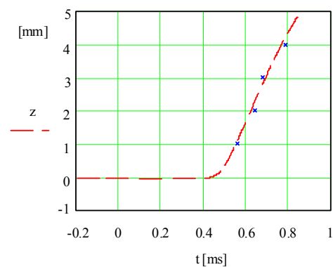
Fig.27. Displacement versus time for W=245J .
