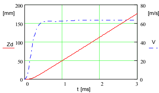
Fig. 6. Displacement and velocity of disc.
