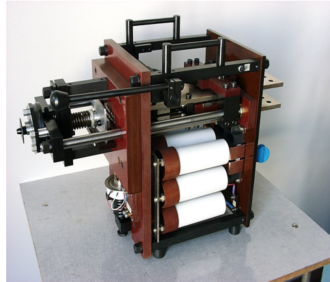
Fig. 2. Physical model of ultra-rapid HB [1].
