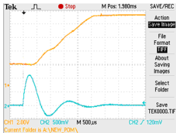
Fig. 20. The oscillogram of the disc displacement and the coil current.
