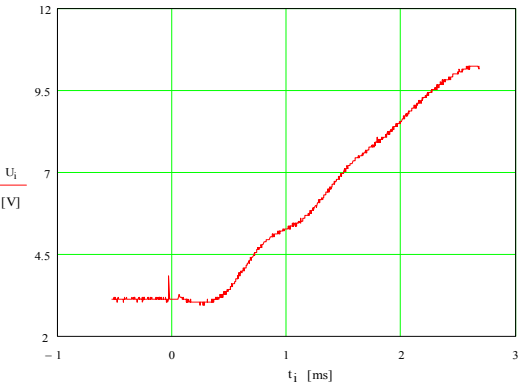
Fig. 23. The U(t) characteristic of optimizer.
